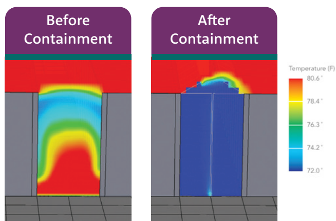
CFD analysis shows a significant reduction in hot air recirculation when aisle-end doors applied in conjunction with Rack Top Baffles at the end of the cold aisle.
