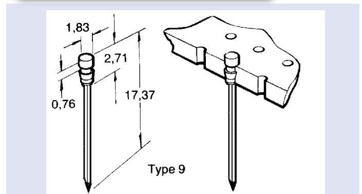
Miniwrap Terminal Pin – Type 9
