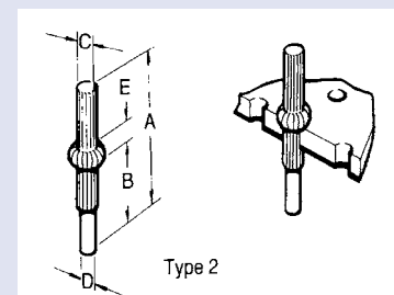
Solder Terminal Pins – Type 2
