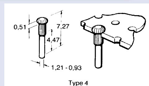
Solder Terminal Half Pins – Type 4
