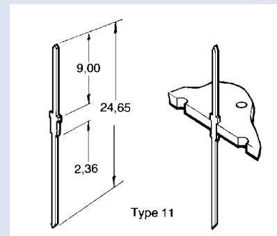
Double Sided Pins – Type 11
