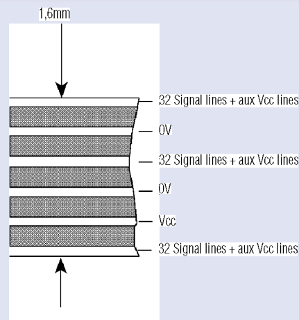
Multilayer uncommitted extender boards
