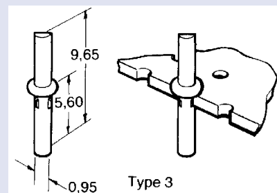
Solder Terminal Pins – Type 3
