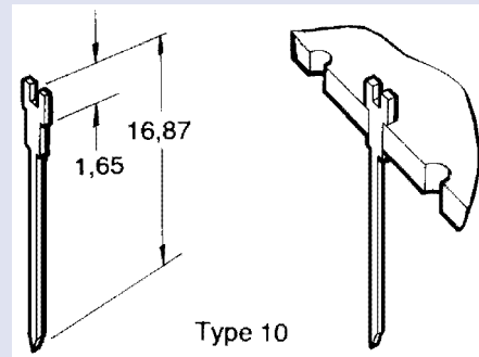
Single Sided Pins – Type 10
