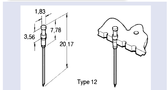
Test Point Pins – Type 12
