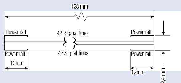
Multilayer Microbus backplanes
